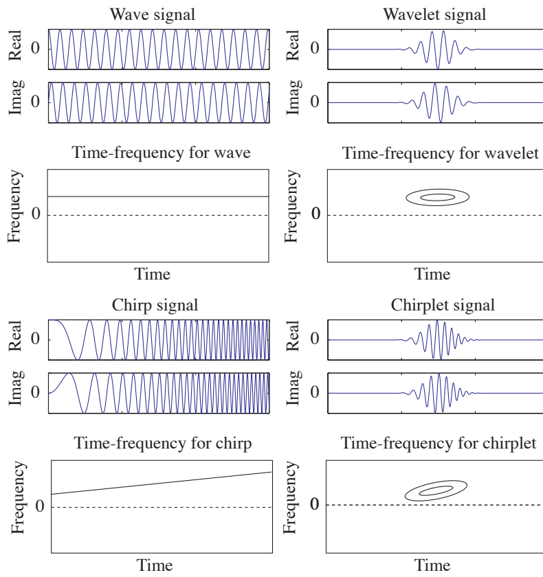
Figure 1: Wave, wavelet, chirp and chirplet.
